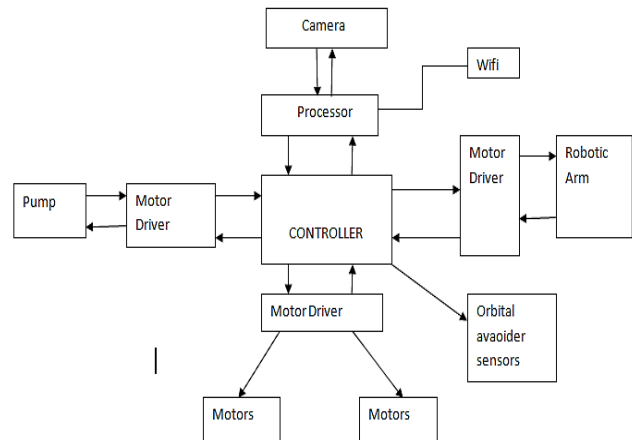
Fig-1: Block diagram for automated ground harvesting machine
