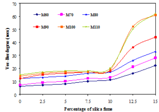
Figure 4 Workability through Vee- bee values
