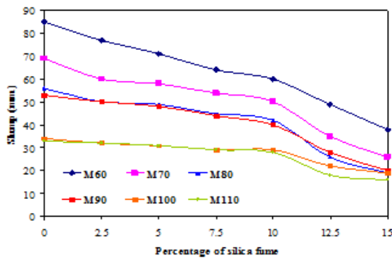
Figure.2 Workability through slump values
