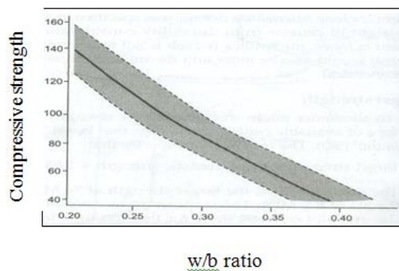
Figure 1 Proposed w/b ratio Vs compressive strength relationship from BIS: 456- 2000
