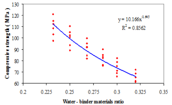
Figure 5 Relationship between compressive strength and water-binder ratio of silica fume-based concrete
