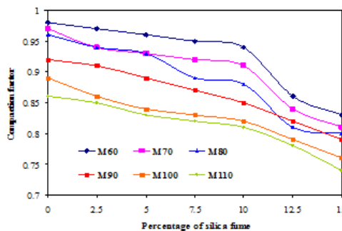
Figure 3 Workability through compaction factor values
